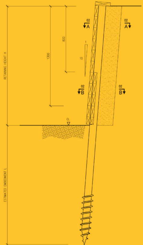
SCREW ANCHOR RETAINING WALL SECTION
