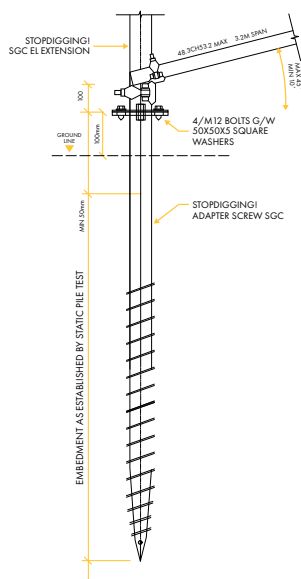
▲ FIGURE 7. BRACED SCREWS WITH SGC EL EXTENSION
