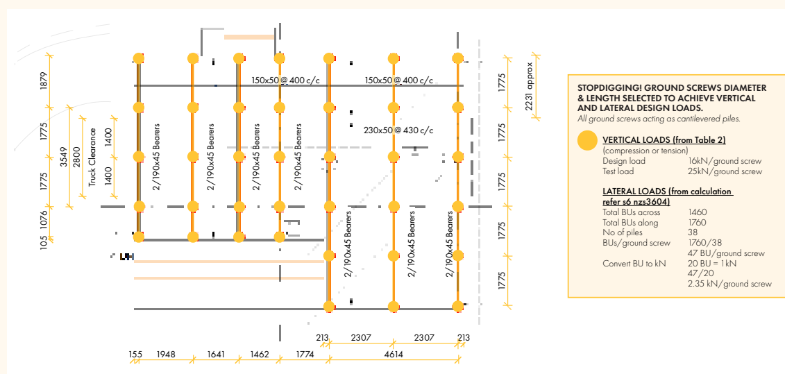
▲ EXAMPLE 1. LEVEL SITE WITH CANTILEVERED PILES
