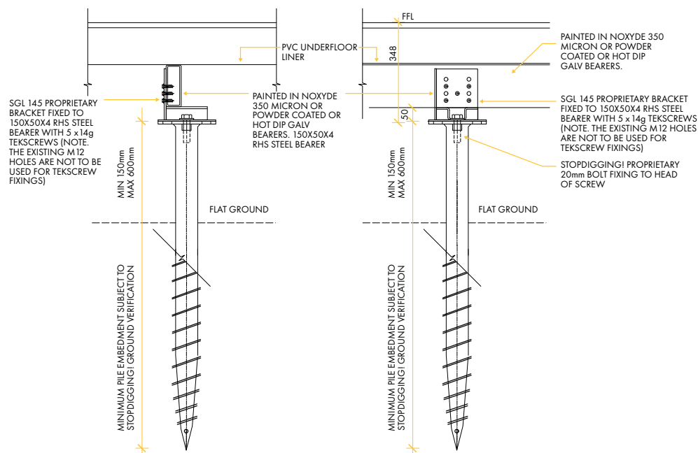
▲ FIGURE 6. SGC ADAPTOR SCREW PILE SGL 145 STOPDIGGING! BRACKET
